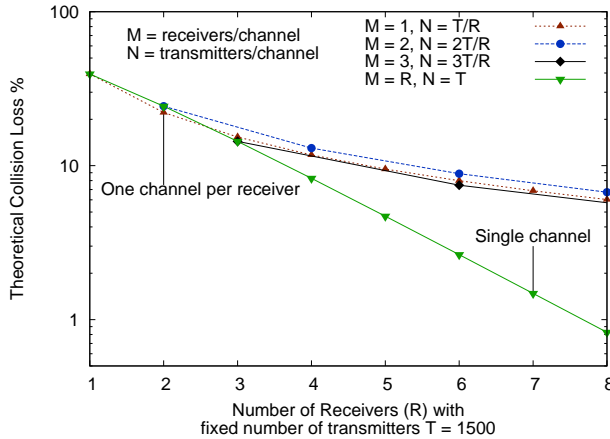
Figure 7: Theoretical packet losses with \alpha = 2.69 , one 300 \mu second transmission per second, and 1500 transmitters, using Equation 2 and P_{capture} from Figure 5 and Equation 3. Once of the number of receivers passes a threshold a single channel is better than using multiple channels.
